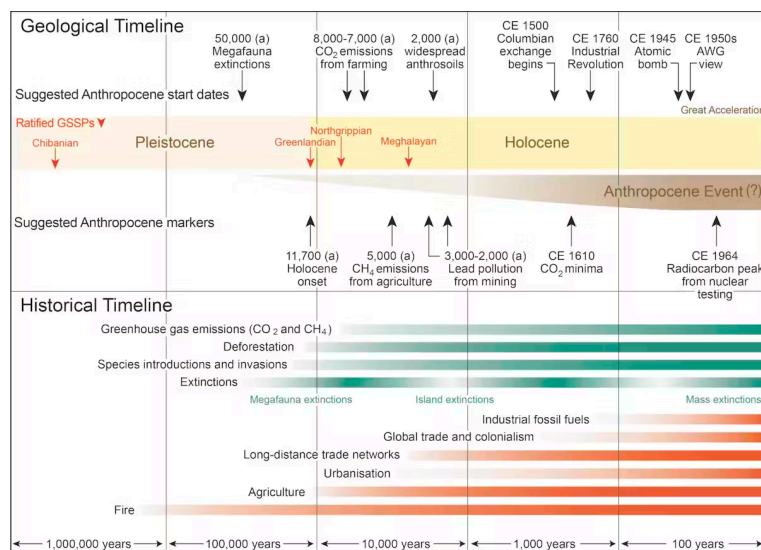
A chart reflecting timing of the ‘Anthropocene Event’ shows how various human activities have affected the planet over millennia in the recent geologic time scale. Click the image to enlarge. Philip Gibbard, et al., 2022
